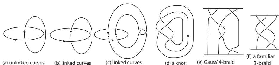
FIGURE 1. Links, knots and braids
