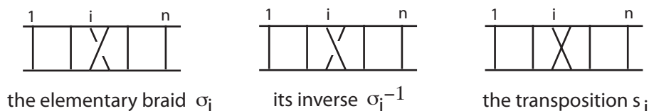
FIGURE 2. Elementary braids and permutations
